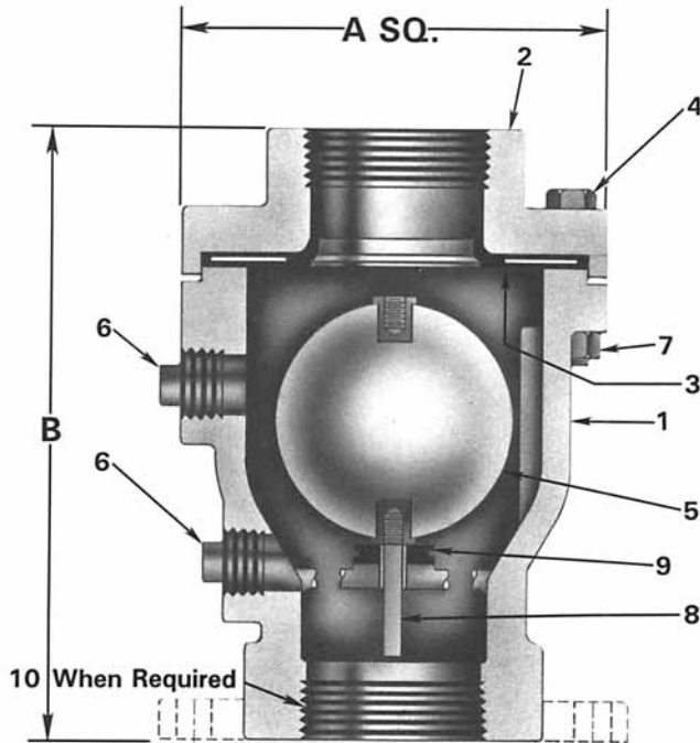
FIG. 930 (4") Flange Dimension Per ANSI B16.1 Class 125 (CL.250 Optional)
